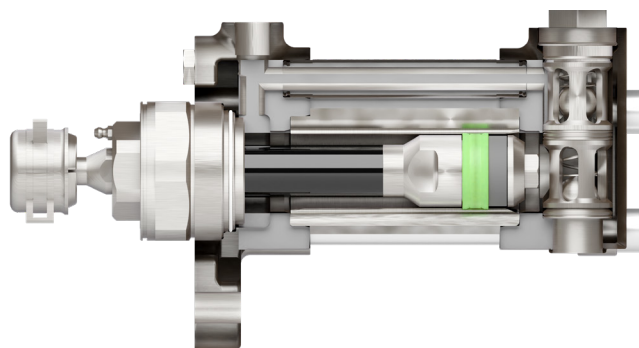
Cutaway of Z-Pump with Elite Technology
